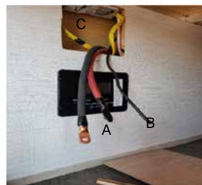
2 | A. 2 gauge inverter cables B. 8 gauge ground cable C. Amp connector
